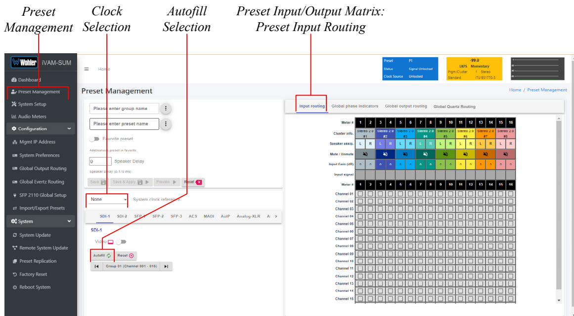
Figure 4-18: Configure Presets
