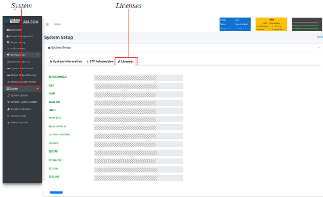
Figure 4-34: Licenses Tab
